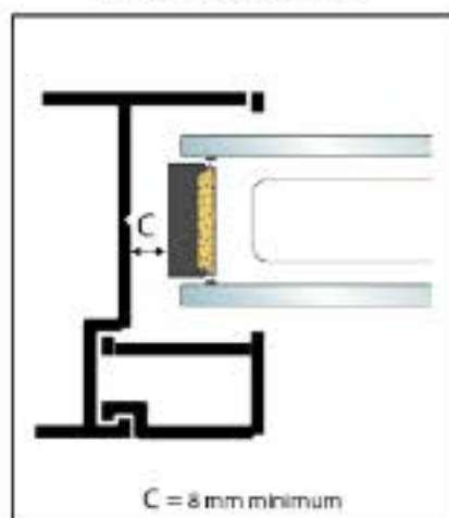
ORIZONTAL SECTION
