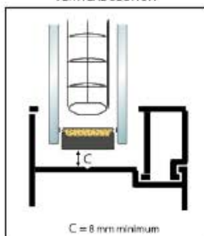
VERTICAL SECTION
